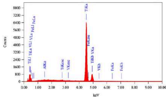
Gambar 1. Hasil Uji EDS sampel ( pre-test )
