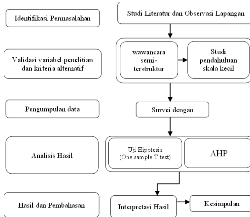
Gambar 6. Alur Penelitian
