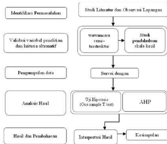
Gambar 6. Alur Penelitian
