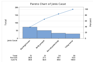
Figure 3. Pareto Diagram
