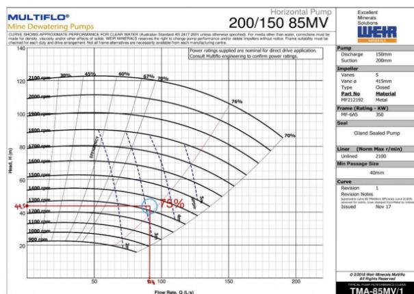
Gambar. 3 Pump curve RF-85MV 92l/s
