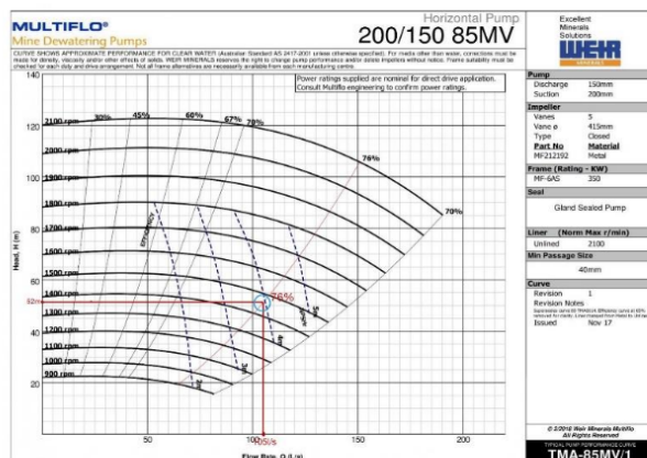
Gambar. 4 Pump curve HY-85MV Boston Timur
