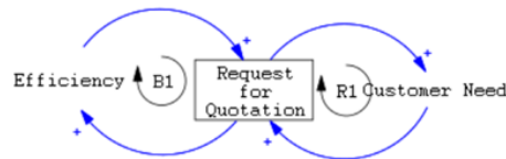
Figure 5. Archetype pattern
