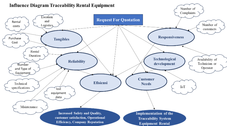
Figure 4. Influence diagram
