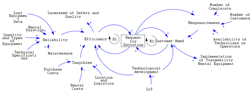
Figure 6. CLD
