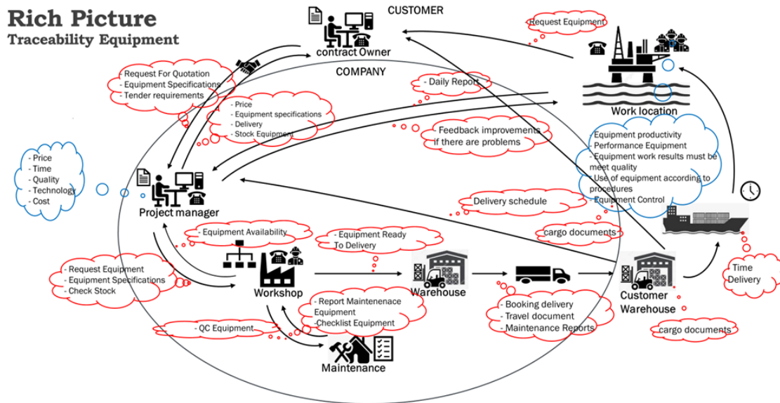
Figure 3. RPD
