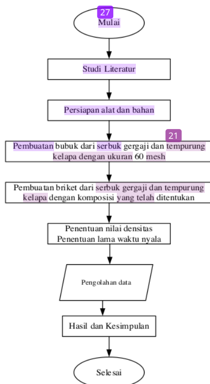
Gambar 1. Flowchart Penelitian
