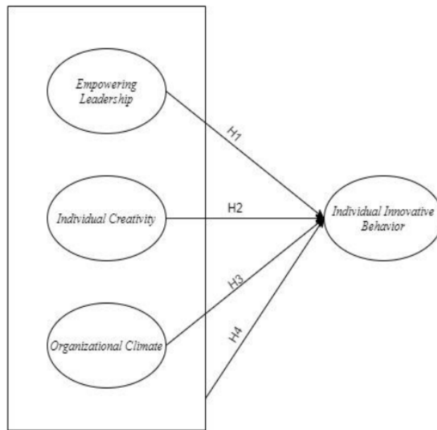
Figure 1. Conceptual Framework
