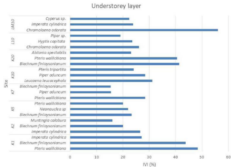
Figure 5. Three species with the highest Important Value Index at understorey layer across asphalt post-mining sites in Buton Island, Southeast Sulawesi Province, Indonesia.
