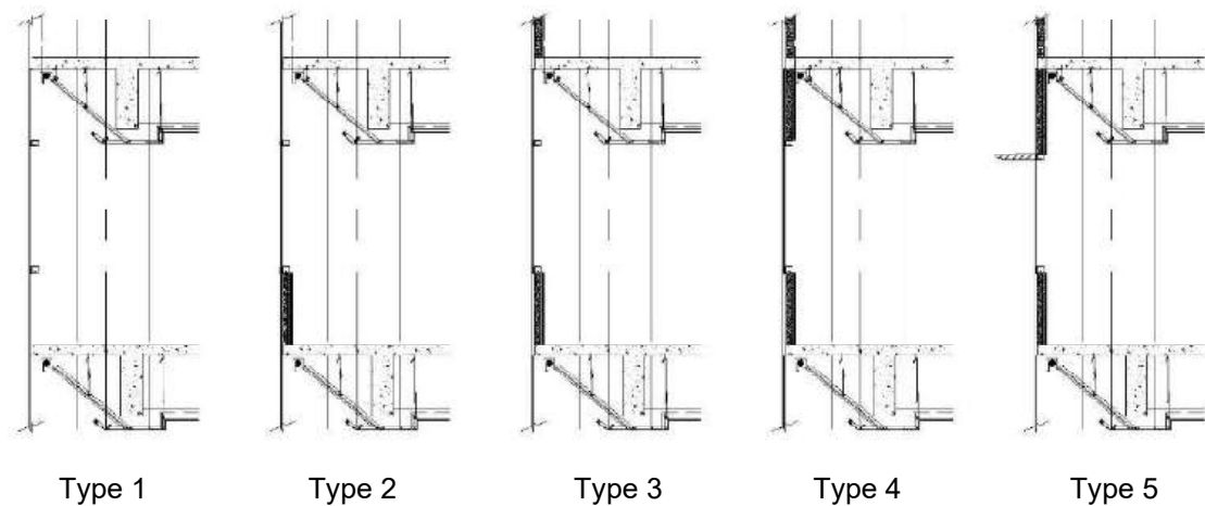
Figure 1. Five varieties of wall systems
