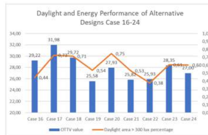
Figure 1. Daylight and Energy Performance of Alternative Design Case no 16-24
