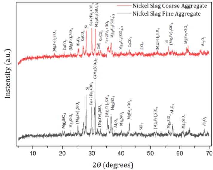
Figure 8 X-ray Diffraction Results of Nickel Slag Aggregate
