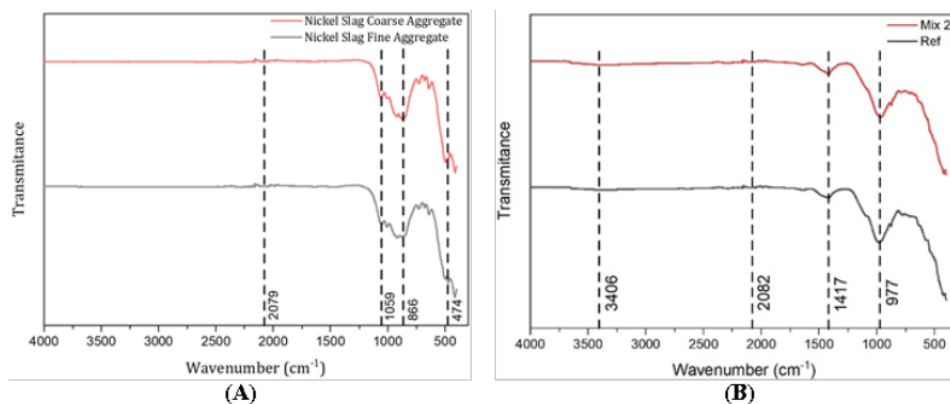
Figure 10 Fourier-Transform Infrared Spectroscopy (FTIR) Results, (A) Nickel slag aggregate, and (B) Concrete from Mix 2 and High-Performance Concrete as Reference (Ref)
