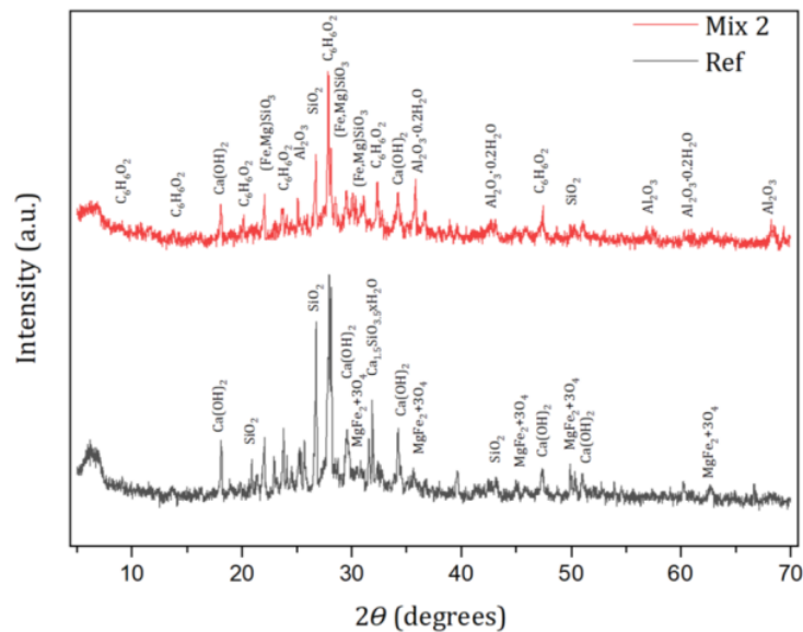
Figure 9 Comparison of X-ray Diffraction (XRD) Results for Concrete Composition Mix 2 and High-Performance Concrete as Reference (Ref)
