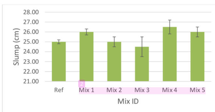
Figure 2 Results of the Slump Test Conducted Using Abrams Cone Apparatus Under Standard Conditions
