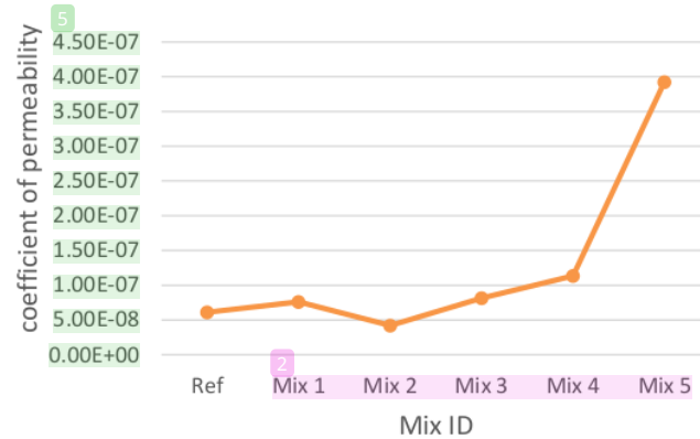
Figure 5 Permeability Coefficient Results Tested Using an Air Permeability Apparatus
