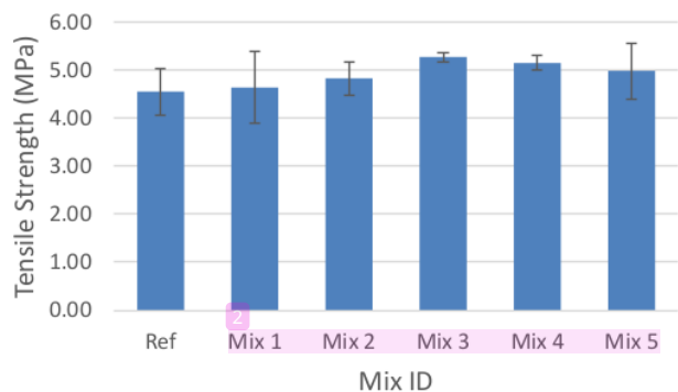
Figure 4 Tensile Strength Results at 28 Days Tested Using a Digital Concrete Compression Machine
