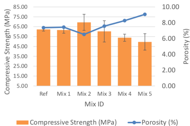
Figure 7 Comparison of Porosity and Compressive Strength
