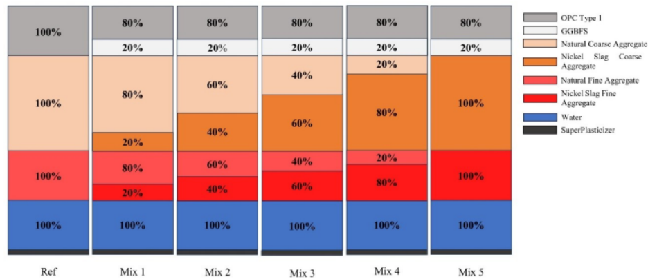
Figure 1 Composition of Concrete Mixes, Including Variations in Binder Proportion (OPC and GGBFS), Aggregate Types (Nickel Slag and Natural Aggregates), and 1% superplasticizer dosage
