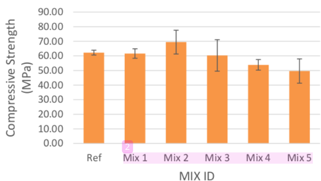
Figure 3 Compressive Strength Results at 28 Days Tested Using a Digital Concrete Compression Machine
