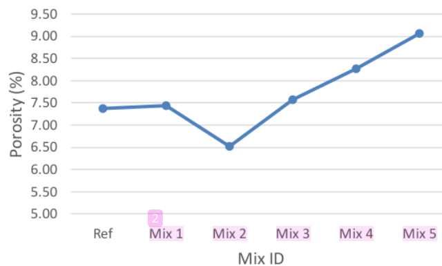
Figure 6 The Results of the Porosity Test Indicate an Increasing Trend Correlated with the Permeability
