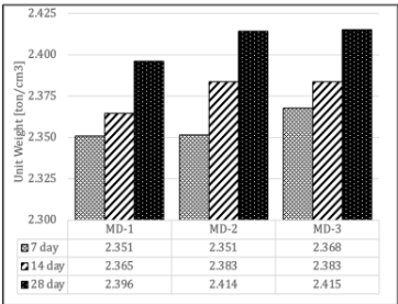
Fig. 3. Unit weight value of the test specimen
