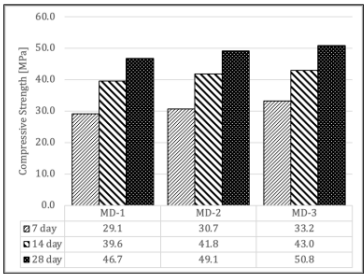
Fig. 4. Compressive strength value of the specimen
