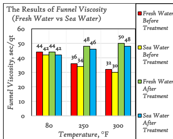
Figure 2. Funnel viscosity measurement results
