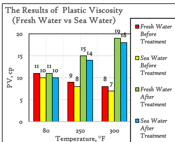
Figure 3. Plastic viscosity measurement results
