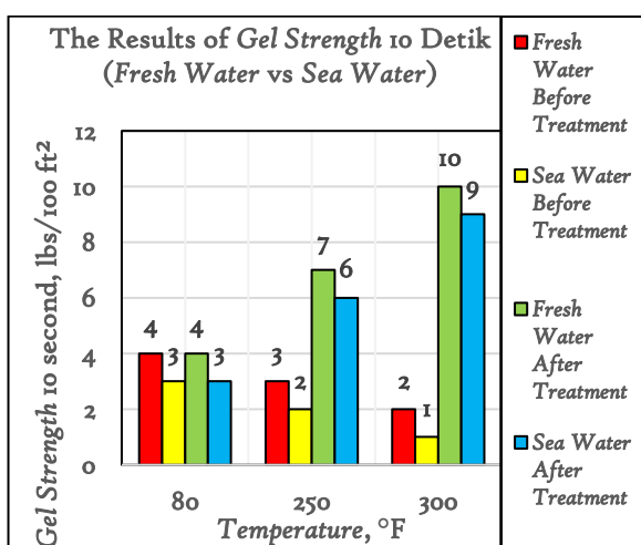
Figure 5. 10 Second gel strength measurement results
