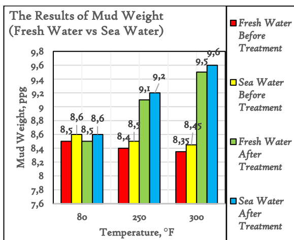
Figure 1. Mud weight measurement Results
