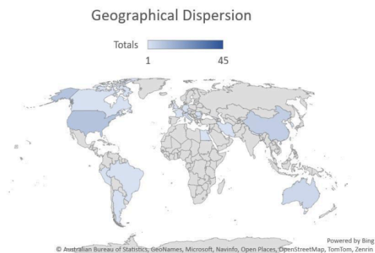
Fig. 3: Map showing the geographical distribution of paper based on contributions from various countries
